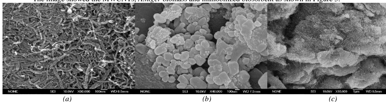
Figure 5. FESEM images (a) A.niger biomass (b) functionalized MWCNTs (c) Immobilized biomass with MWCNTs
